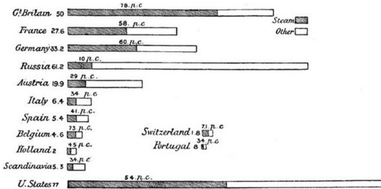
STEAM AND OTHER POWER IN DIFFERENT COUNTRIES.
